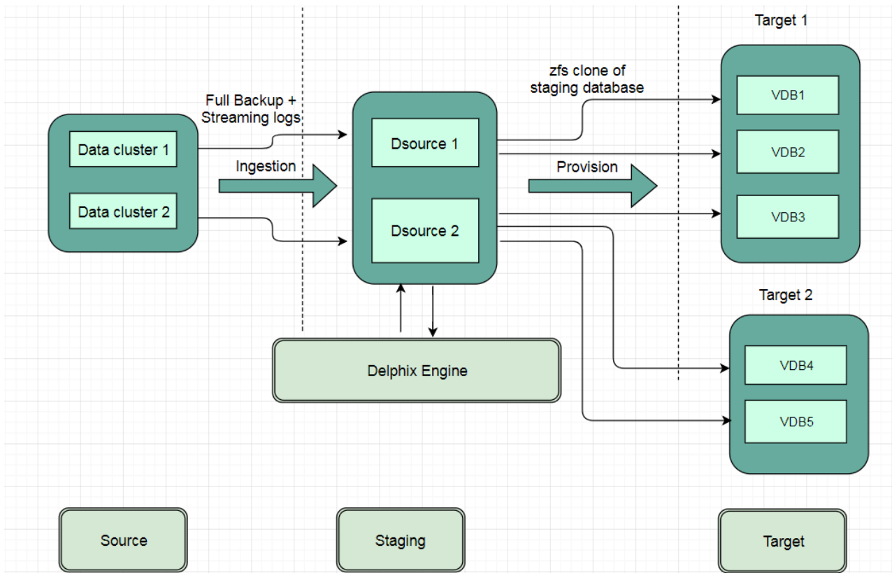
Block Diagram of Linking Architecture Between PostgreSQL Environments and the Delphix Initiated Backup Platform.
