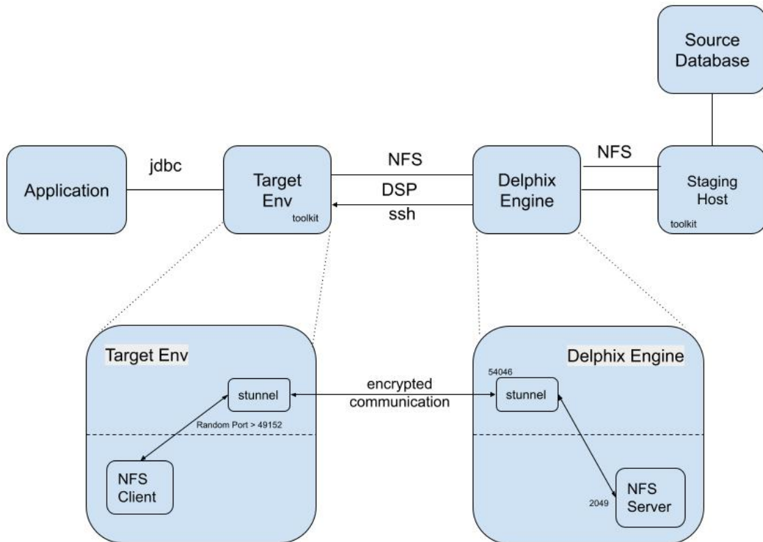
2 Image 1. NFS - Architecture
