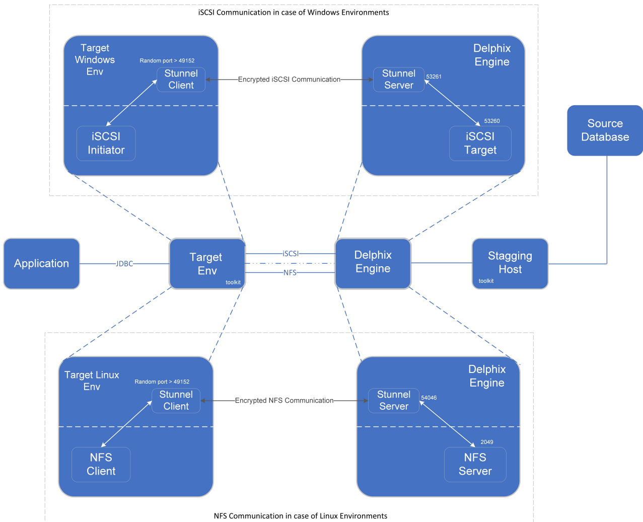
2 Image 1. NFS - Architecture
