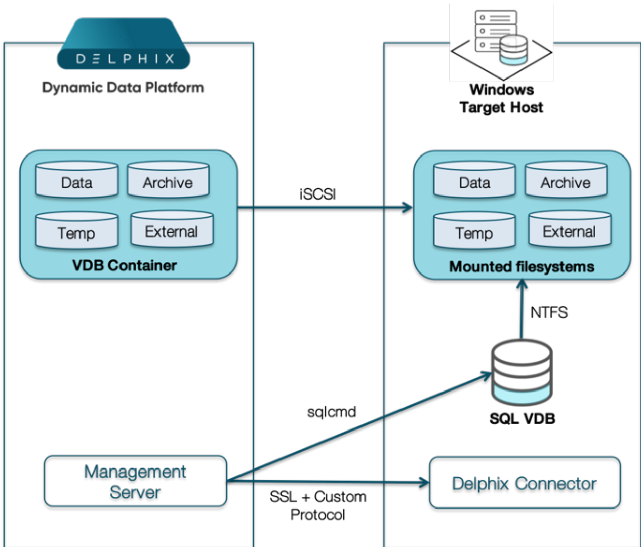
Block diagram of SQL server provisioning architecture
