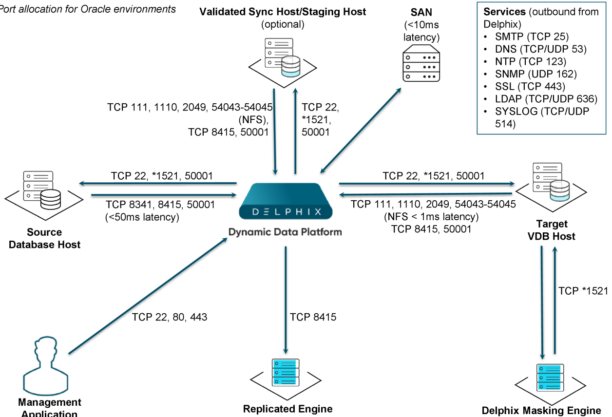
Port allocation for Oracle environments
